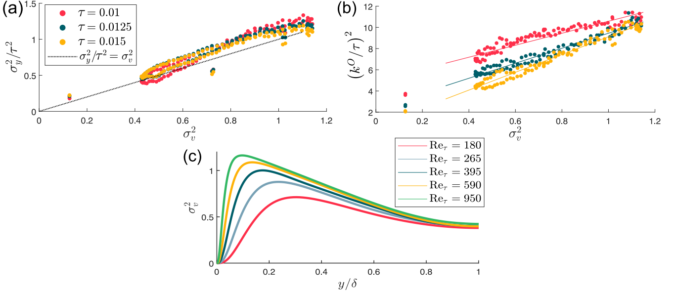
FIG. 2. (a) Variance of the position of particles released from each node and divided by \tau^2 , plotted against the velocity variance at the release location, at Re_\tau = 950 . (b) Squared outgoing degree (k^O/\tau)^2 , averaged over different realizations at Re_\tau = 950 and divided by \tau^2 , versus the velocity variance. (c) Wall-normal velocity variance profiles across the channel half-height.
