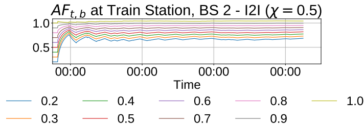
Figure 10: AF_{t,b} for a micro cell BS of the Train Station area, with \chi=0.5 , varying AF_{sleep}
