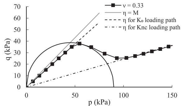
Fig. 13. Transition from the stress path \eta tending to K_0 to the obliquity \eta tending to K_{nc} when the soil yields in the p - q plane.
