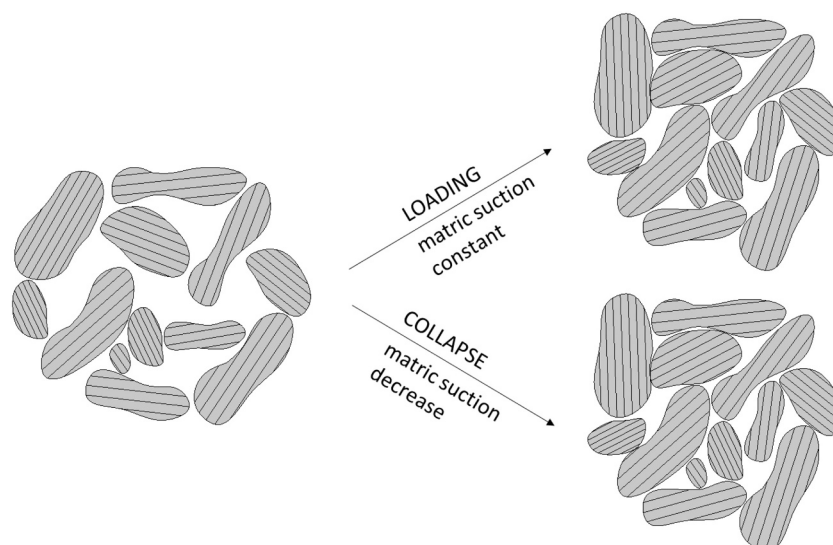
Fig. 2. Microstructure evolution of a partially saturated soil with open fabric subjected to mechanical loading or to wetting.
