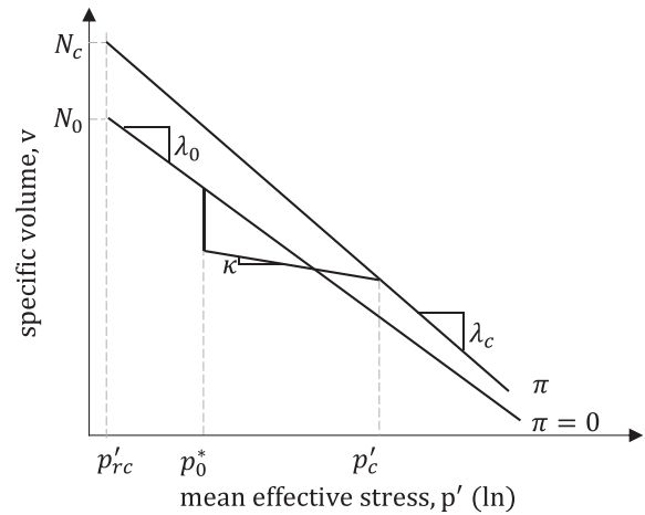
Fig. 6. Compression curves for soil saturated with distilled water ( \pi = 0 ) and for soil saturated with a saline solution. Relationship between preconsolidation stresses p_0^* and p'_c .
