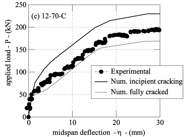
FIGURE 10 Comparison between the experimental data and the results of the three-stage model: (a) P - \eta curves of the beam 12-70-A; (b) P - \eta curves of the beam 12-70-B; (c) P - \eta curves of the beam 12-70-C
