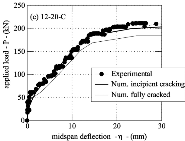
FIGURE 9 Comparison between the experimental data and the results of the three-stage model: (a) P - \eta curves of the beam 12-20-A; (b) P - \eta curves of the beam 12-20-B; (c) P - \eta curves of the beam 12-20-C
