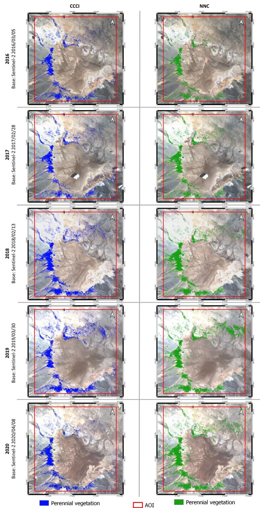
Figure 7. Results of the MD supervised classification for the multi-temporal CCCI and of the SAM supervised classification for the NNC images. Reading the figure vertically, changes over time of the perennial vegetate areas are visible.
