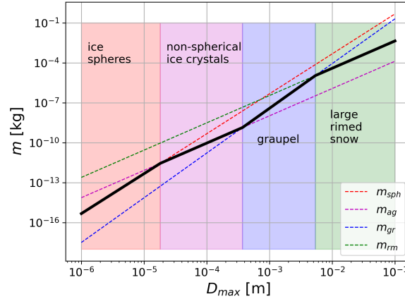
Figure 1. Mass–size parametrization of Morrison and Grabowski for rimed aggregates. The different colors correspond to the size ranges where a specific power law formula is used: red for small solid ice spheres, magenta for non-spherical ice crystals, blue for fully rimed snow, green for aggregates that are not completely filled with rime.
