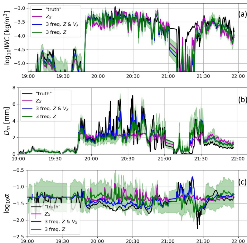
Figure 4. The results of different microphysical retrieval along the validation flight. The black line shows the snow microphysical properties estimated derived from the PSD measurements, Nevzorov probe and radar data. The green, blue and magenta lines correspond to the retrievals based on the triple frequency reflectivity, triple frequency reflectivity with the mean Doppler velocity at the X-band and the algorithm based on the X-band reflectivity only, respectively. The green shading shows the uncertainty of the triple-frequency retrieval.
