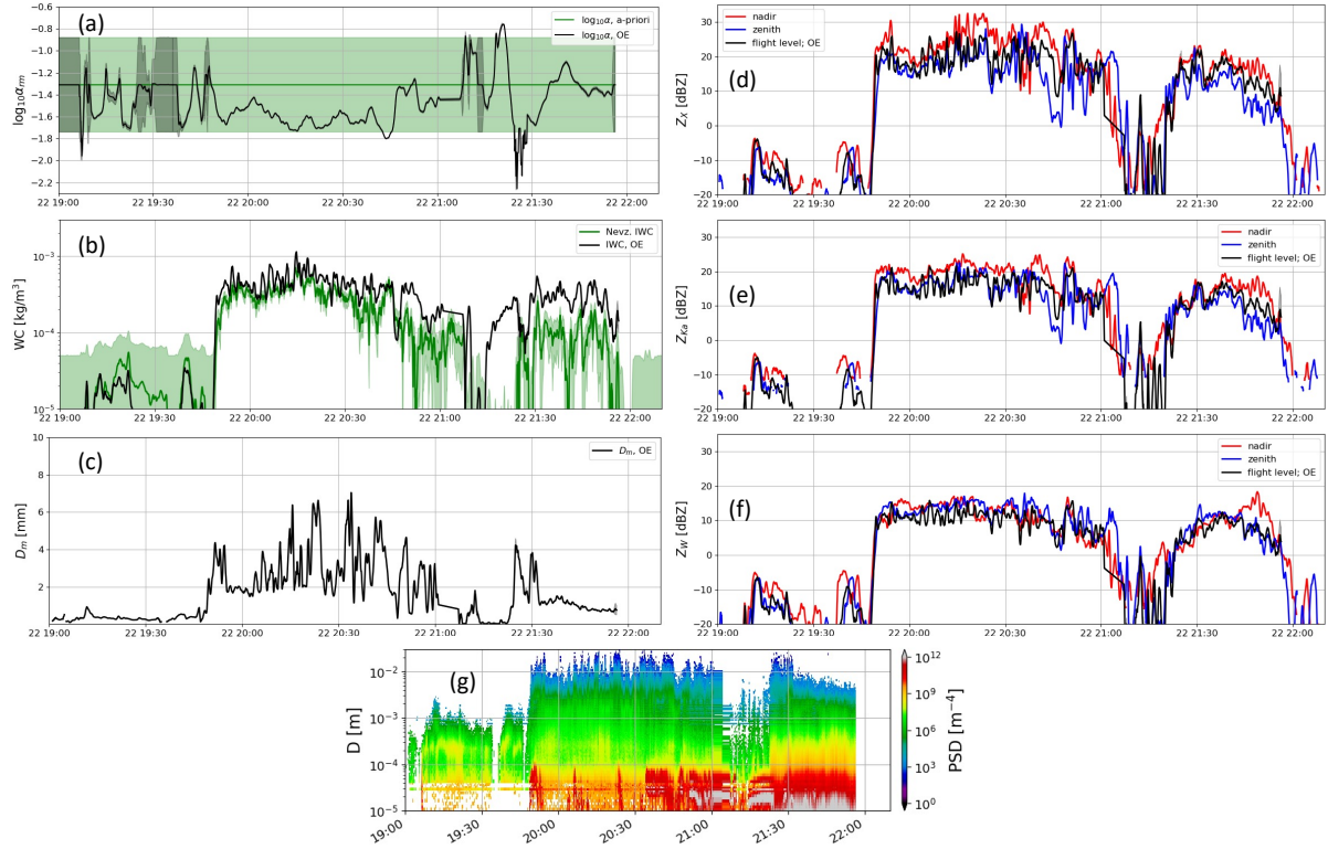
Figure 3. The estimates of the microphysical properties of snow and the radar reflectivity at the flight level. Panel (a) shows the retrieved degree of riming in black and its prior estimate in green. The retrieval is based on the data from triple frequency radar, Nevzorov probe and PSD measurements. Panel (b): the estimated IWC (black) and Nevzorov probe data (green). Panel (c): the estimated mean mass-weighted diameter of snow. Panels (d,e,f) show the reflectivity at the X-, Ka- and W-band, respectively. The red (blue) line shows the measurements below (above) the plane while the black line is the estimate at the flight level that is in agreement with the microphysical properties shown on the left and the collected PSD data (panel g). Shading represents the uncertainty of each estimate.
