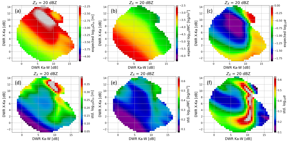
Figure 2. The expected values of \log_{10} D_m , \log_{10} IWC , \log_{10} \alpha_{rm} in the DWR_X-Ka-DWR_{Ka-W} for Z_X = 20 dBZ. This inverse model is derived from the in-situ airborne PSD measurements during MC3E, IPXEx, OLYMPEX and HAIC/HIWC campaigns.
