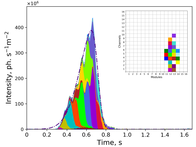
Fig. 15. Light curve of the meteor event TUS170318b and its Skew Gaussian approximation. Inset: pixel map with hit pixels.
