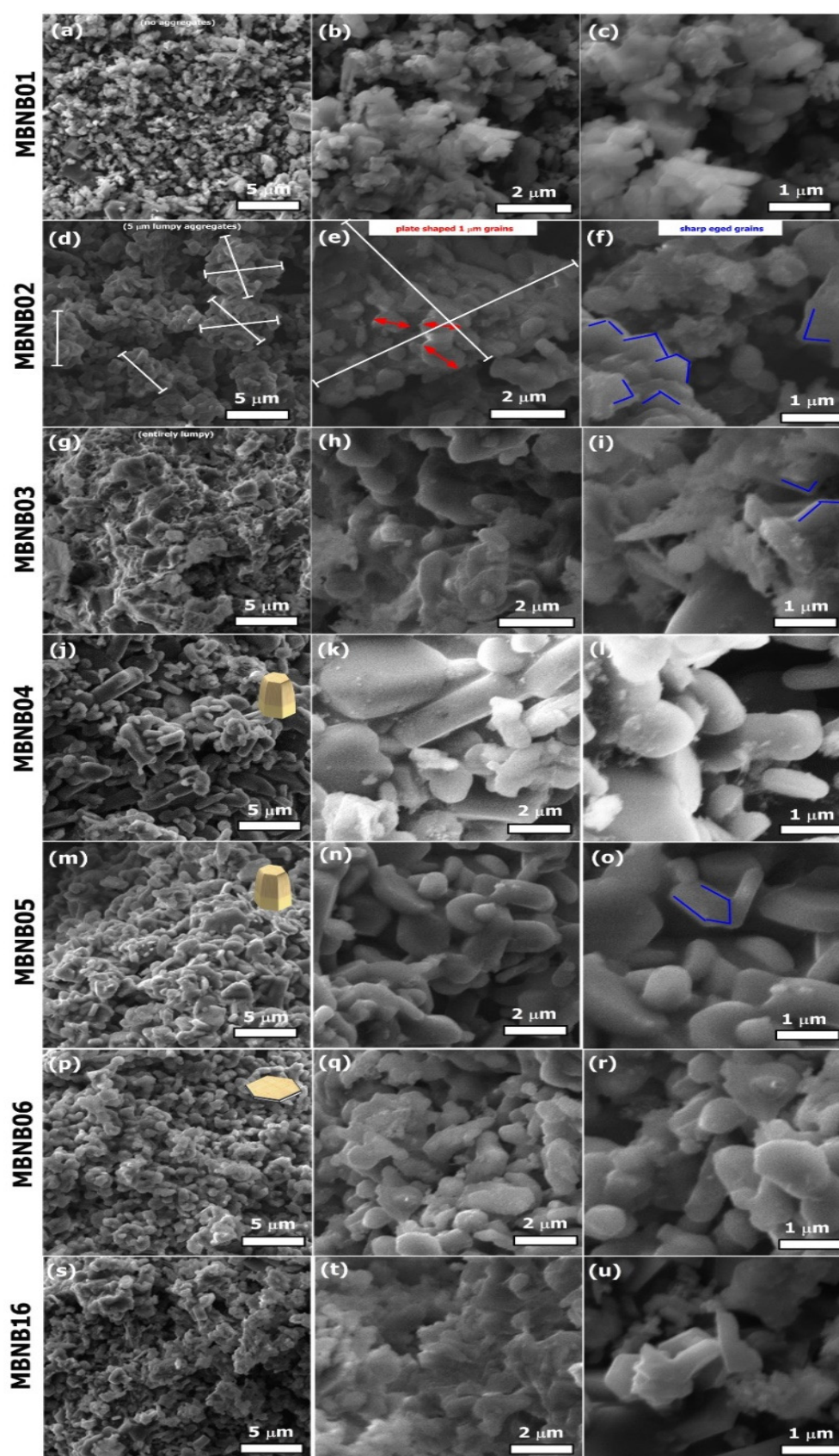
Figure 3. SEM images of the \text{MgB}_2 powders. Images of each row correspond to the sample indicated on the left (see Table 1). The three columns correspond to a magnification of 10 k \times , 30 k \times , and 50 k \times , respectively.
