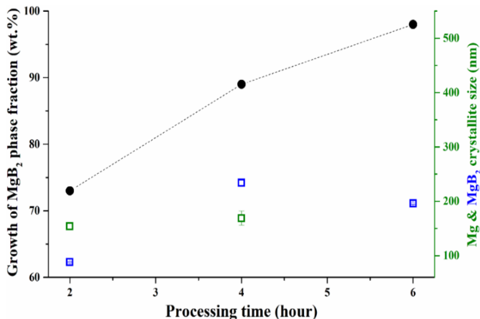
Figure 2. Evolution of the \text{MgB}_2 production versus synthesis duration for T = 800 °C and Mg:B stoichiometric ratio equal to 1.4:2. Black solid circles represent the \text{MgB}_2 percentage weight fractions, and green and blue void squares are the Mg and \text{MgB}_2 crystallite sizes, respectively.
