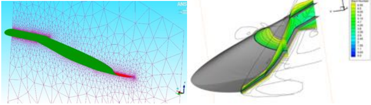
Fig. 8. Grid and Mach 3D contour at M=8
