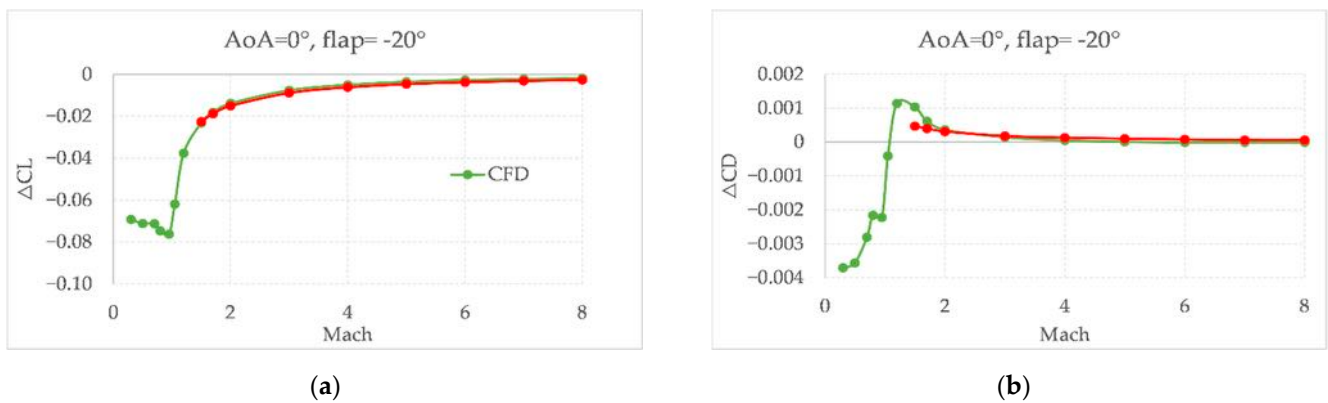
Figure 12. \Delta C_L (a) and \Delta C_D (b) due to the flap effect at \alpha = 0^\circ and flap = -20^\circ . Compared with SIM method in supersonic regime.
