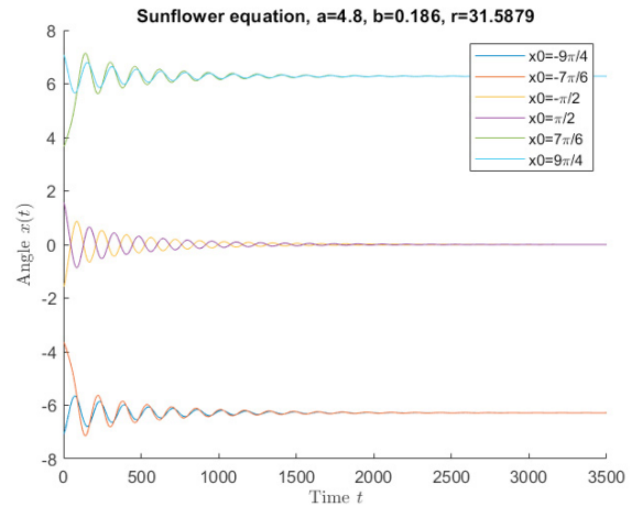
Fig. 2. Solutions converging to equilibria ( r < r_+ ).
