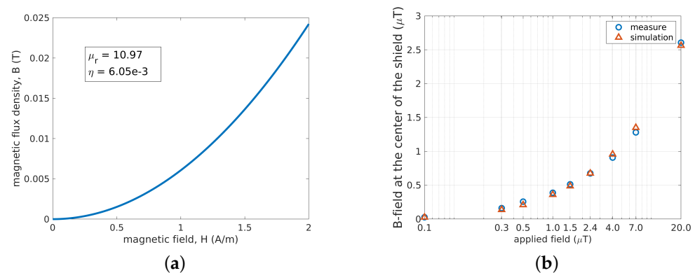
Figure 6. B(H) curve in the Rayleigh region obtained with the identification procedure (a). Comparison of measured and simulated magnetic flux density at the center of the shield for different external field values (b).
