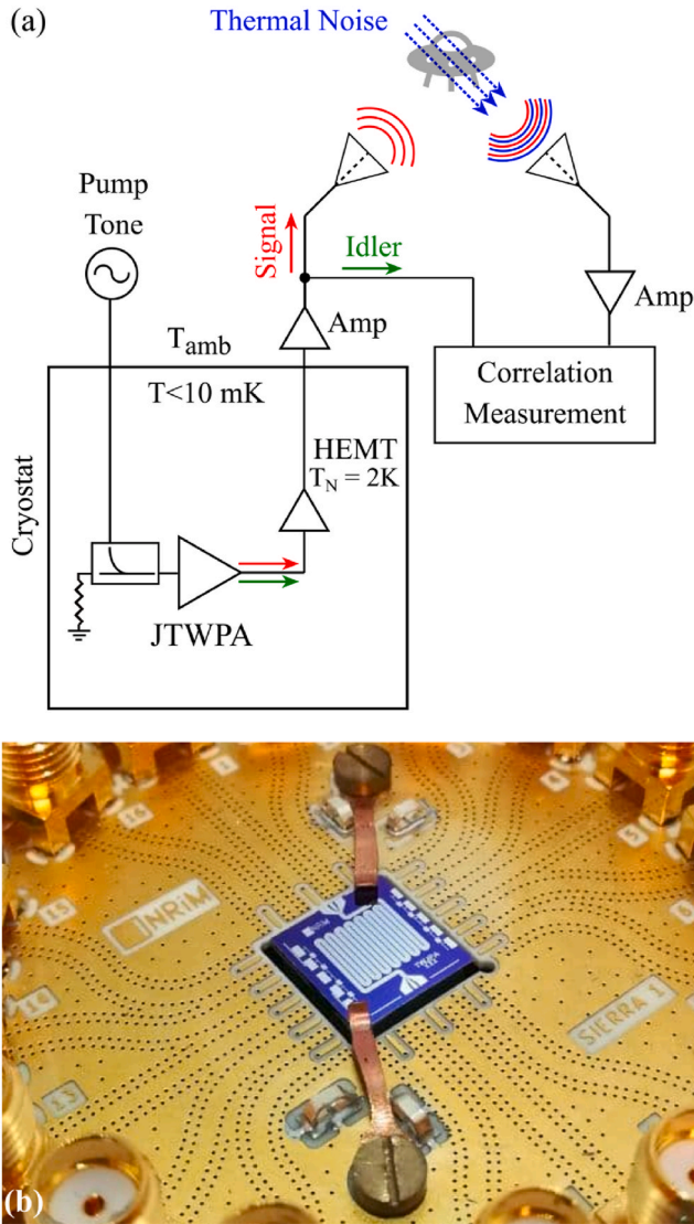
Fig. 2. (a) Schematic representation of a MQI protocol that exploits a Josephson metamaterial, hosted in a cryogenic environment, as a source of two-mode squeezed vacuum states for the detection of low-reflectivity targets at room temperature. (b) Micrograph of a typical Josephson Traveling Wave Parametric Amplifier.
