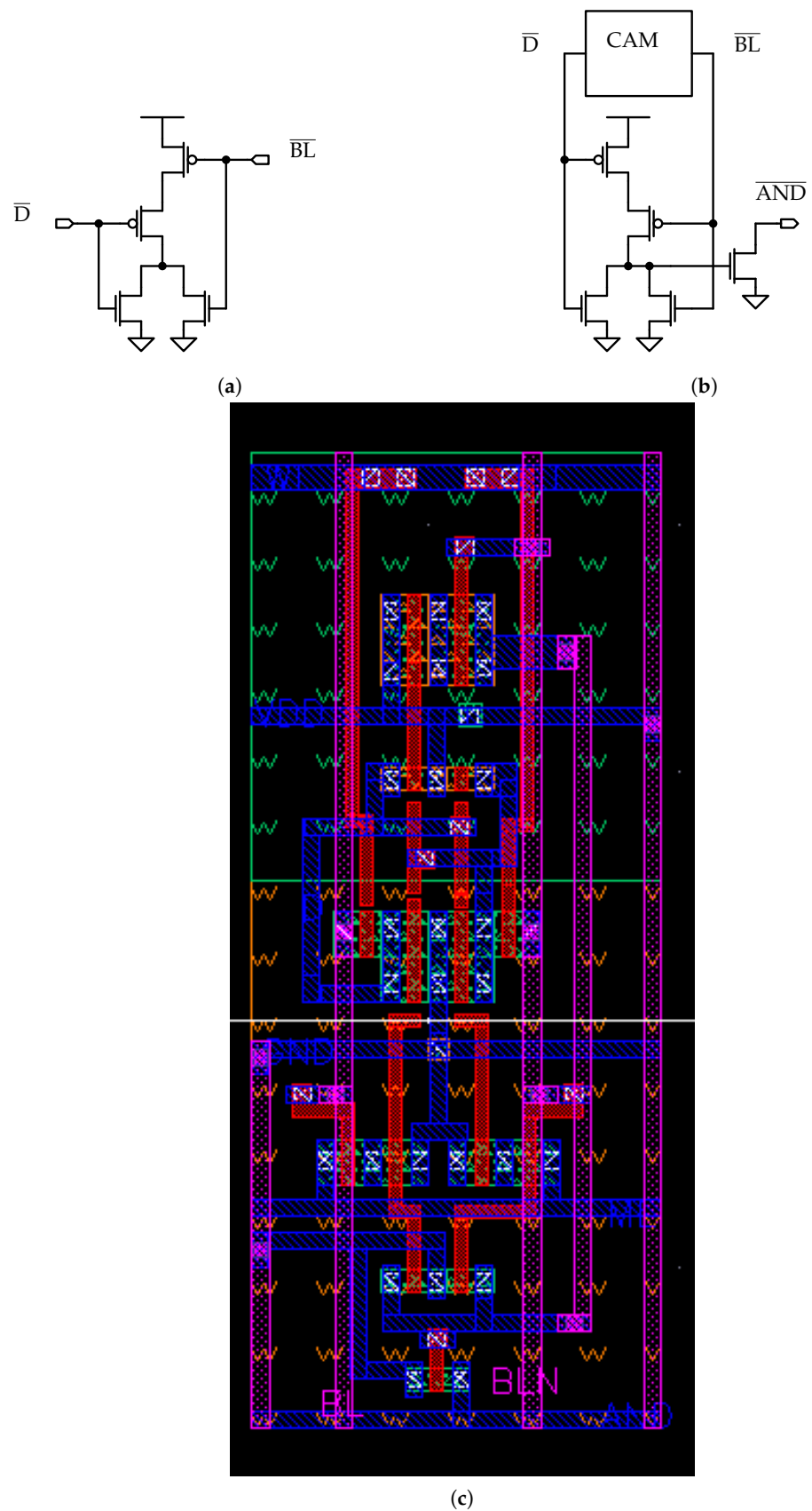
Figure 10. The static AND gate and memory cell. (a) The static CMOS AND gate. (b) The memory cell that embeds the static AND gate. (c) The cell layout.
