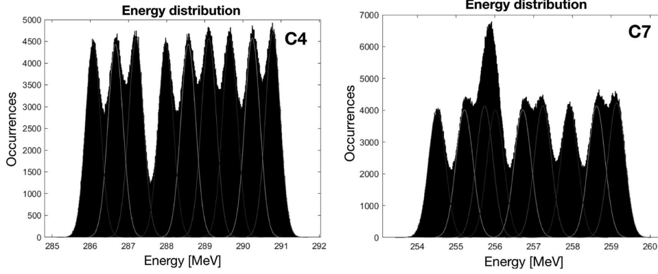
Fig. 2. – Kinetic energy distributions of DCE ejectiles for the reaction ^{130}\text{Te}(^{20}\text{Ne}, ^{20}\text{O})^{130}\text{Xe} with the C4 prototype (left) and ^{116}\text{Sn}(^{18}\text{O}, ^{18}\text{Ne})^{116}\text{Cd} with the C7 prototype (right).
