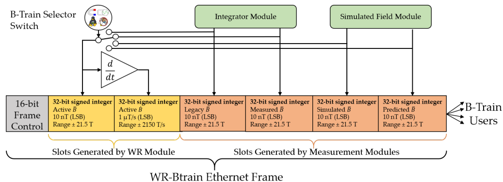
Figure 14. A functional diagram of the broadcast White Rabbit Ethernet frame.
