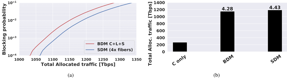
Fig. 2. (a) Total allocated traffi versus BP with BDM and SDM upgrades and (b) allocated traffic multiplicative factor for BDM and SDM comparing with C-band only scenario.
