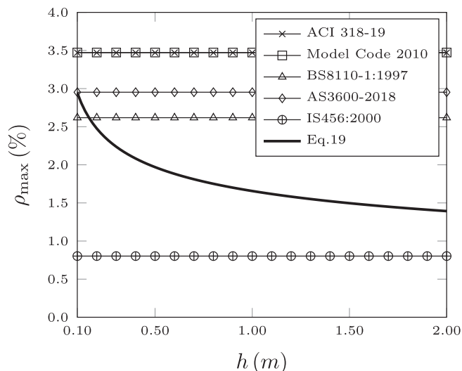
FIGURE 12 Comparison between different maximum reinforcement provisions
