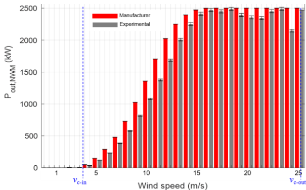
Figure 7. Turbine #1 - NWM corrected results (grey bars) and manufacturer power curve (red bars).
