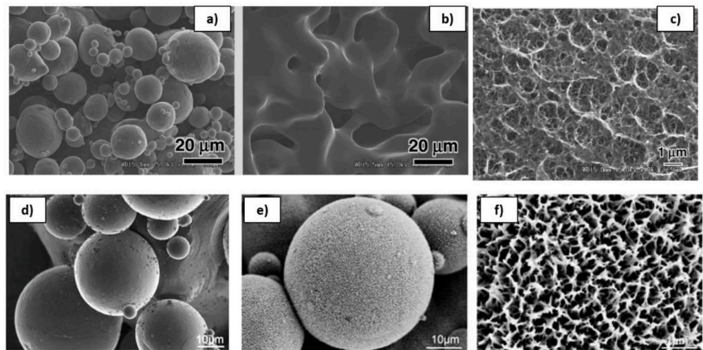
Figure 2. Surface morphology of bare and surface treated AM Ti-based materials. (a) Unmelted particles on SLM Ti; (b) thermally treated (1300 °C) SLM Ti with disappearance of unmelting particles, and (c) nanotexture on SLM Ti after high temperature thermal treatment, chemical, and heat treatment, reprinted from [23] with Elsevier’s permission; (d) unmelting particles on the surface of SLM Ti with bulbous-stripy structure, (e) detail of the microtopography, and (f) nanotexture obtained by hydrothermal treatment, reprinted from [29].
