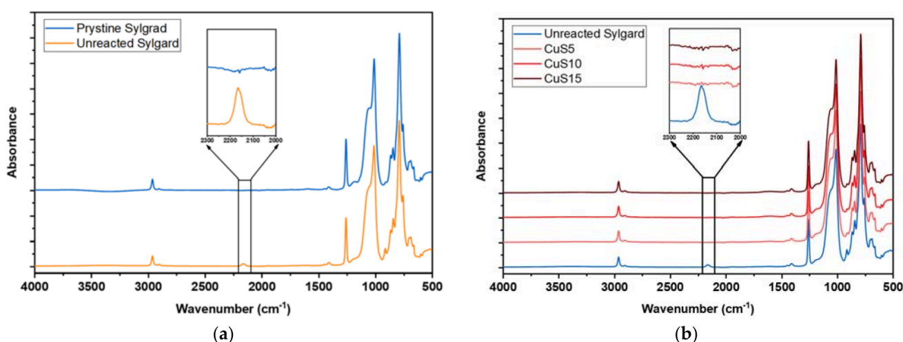
Figure 1. ART-FTIR spectra; (a) spectra of Sylgard pristine formulation (Entry 1; Table 1) before (orange curve) and after (blue curve) thermal curing at 150 °C. zoom of the Si-H peak at 2160 cm -1 in the insert of the graph; (b) spectra filled Sylgard formulation containing spheroidal Cu (Entry 2, 3, 4; Table 1), before (blue curve) and after (red curves) thermal curing at 150 °C. Zoom of the Si-H peak at 2160 cm -1 in the insert of the graph.
