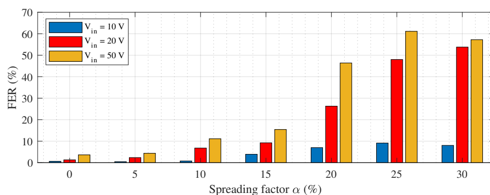
Figure 8. The PLC channel FER evaluation in the case of SSM EMI with several amplitudes and spreading factors \alpha .
