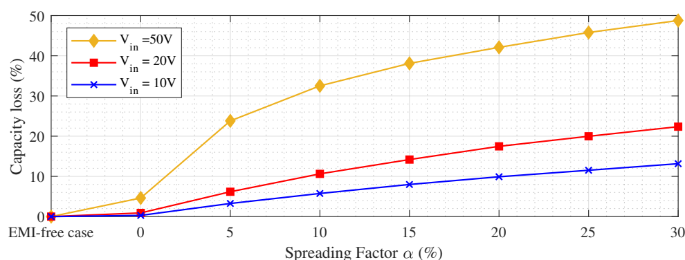
Figure 10. The PLC channel capacity loss in the case of several values of spreading factor with the change in input voltage amplitude of the converter.
