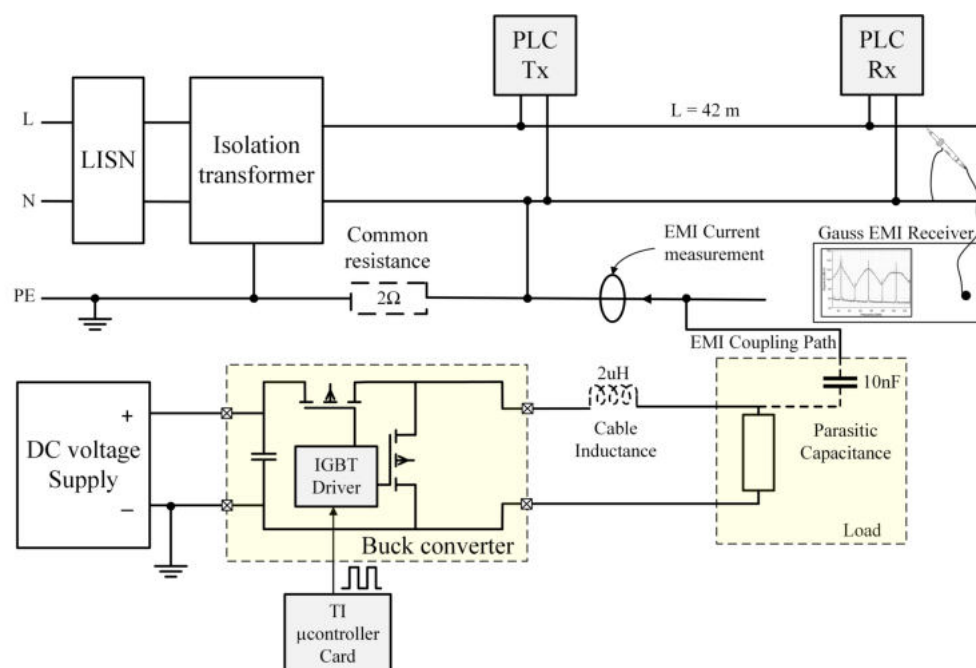
Figure 3. Connection diagram of the system.
