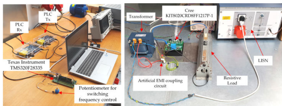
Figure 4. Setup testbed.
