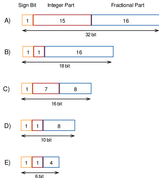
Fig. 5: Fixed-Point Data Representation.
