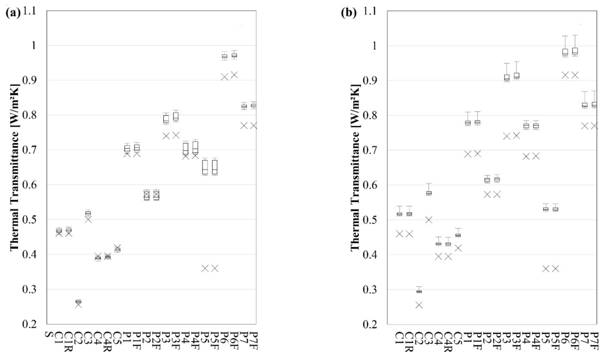
Figure 7. Box plots: Thermal transmittance values of the wall, U [ W/m^2K ], in the winter period (October–April) in Monfero (a) and Turin (b).
