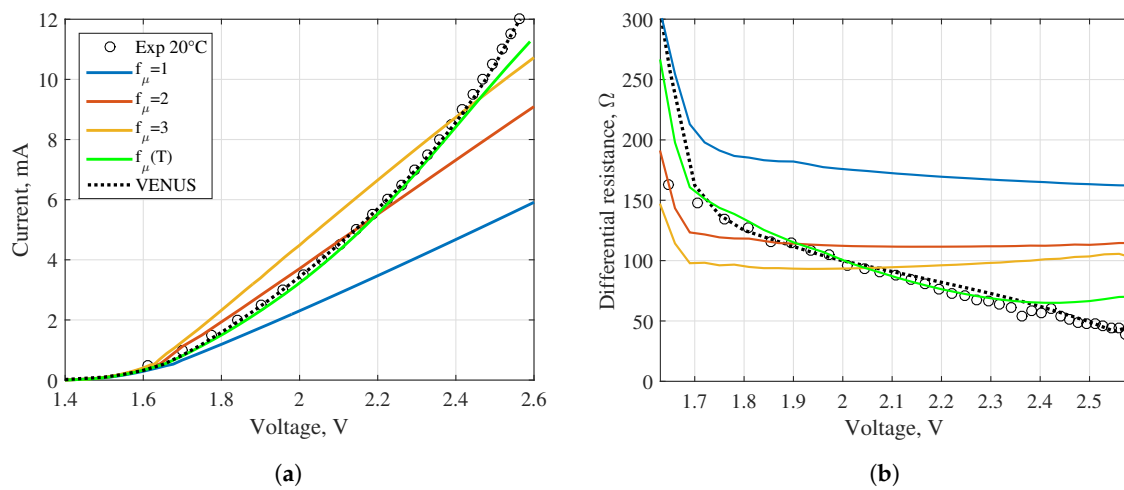
Figure 7. (a) Experimental and VENUS current voltage (I-V) characteristics ( T_{amb} = 20^\circ\text{C} ) compared with the 1D model, with mobility factors that modify the 3D values. (b) Corresponding differential resistances compared with VENUS and experimental result.
