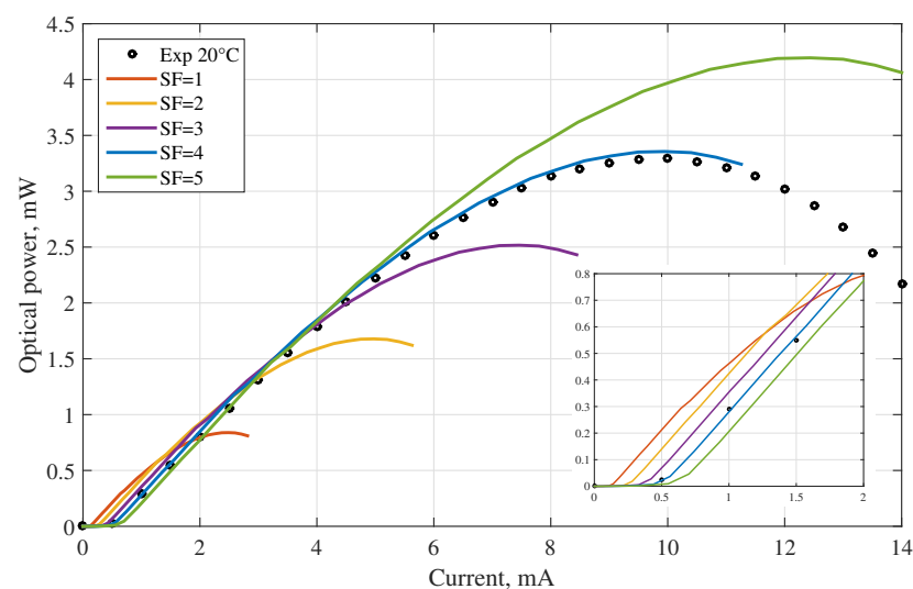
Figure 8. Experimental light-current (L-I) characteristics ( T_{amb} = 20^\circ\text{C} ) compared with the 1D model, with different size factors (SF). The inset shows the threshold behavior.
