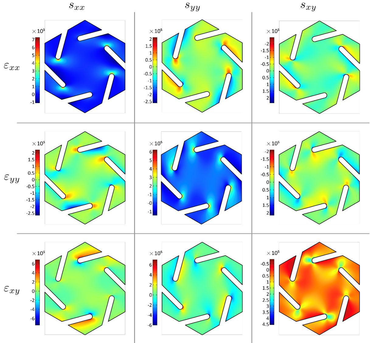
Fig. B.1: Non-hierarchical geometry. Local stress fields in the unit cell for different applied average strains as in Fig. 2 and Tables A.1 and A.2.
