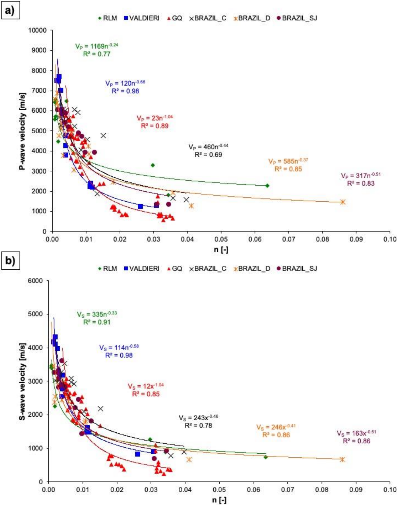
Figure 4: Relationship between P-wave (a) and S-wave (b) velocity and porosity for the studied samples.
