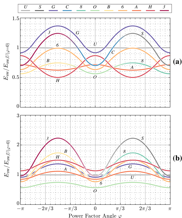
Fig. 14 Switching losses in a area ① and b area ②, normalized with respect to the switching losses of sequence U at \varphi = 0 in each area. The analytical derivation of these expressions is provided in Appendix 2. Some modulation strategies, i.e. S-C-3 , B-O-8 in area ① and S-3 , B-8 in area ②, yield identical switching losses and are thus superimposed. The highest switching loss values are encountered in area ②, since the V_{Z1} \leftrightarrow V_{Z2} lossless transitions (i.e. V_{sw} = 0 ) are replaced by V_{L1} \leftrightarrow V_{L2} (i.e. V_{sw} = V_{dc} ). Therefore, all sequences which include these transitions are strongly favored or penalized depending whether the SNPCC is operating in area ① or area ②, respectively. The switching loss maxima in correspondence of \varphi = \pm\pi/2 are directly related to the 2-L inverter devices, since the two 30^\circ switching windows of each bridge-leg (see Fig. 4a) become aligned with the respective phase current positive and negative peaks, thus maximizing the averaged switched current
