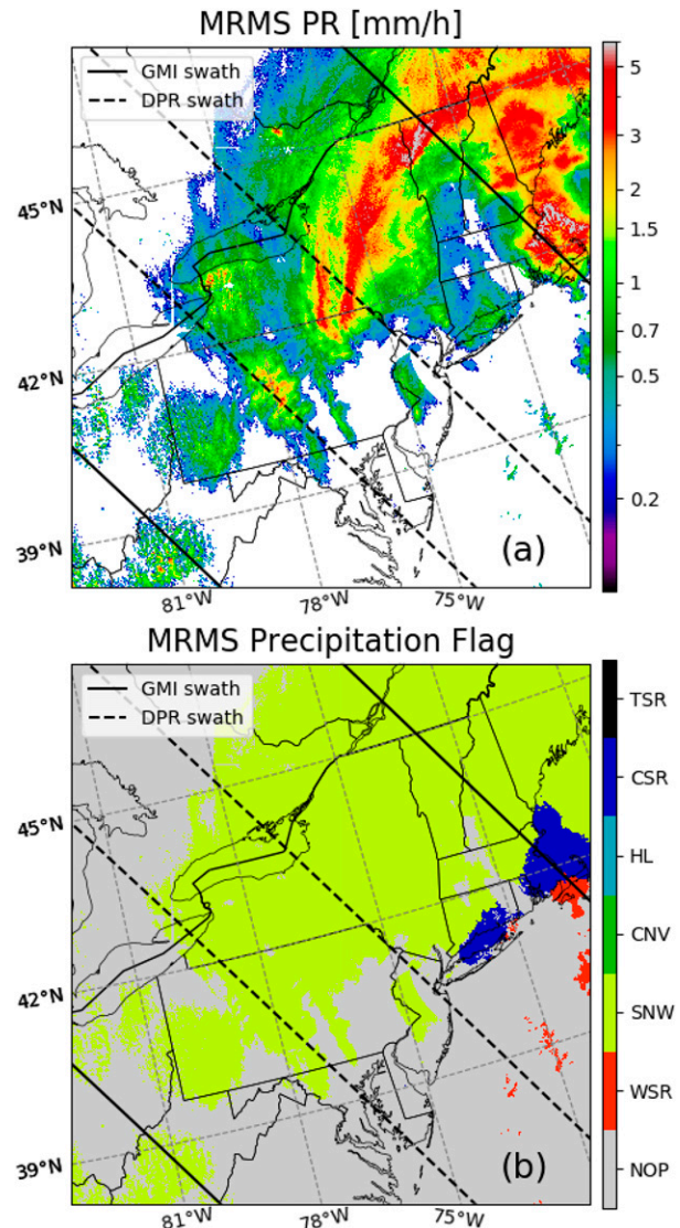
FIG. 2. An example of MRMS products over the northeast United States at 0002 UTC 14 Mar 2017. (a) Instantaneous precipitation rate (PR) derived every 2 min from the radar measurements. (b) Precipitation phase flag (NOP—no precipitation; WSR—warm stratiform rain; SNW—snow; CNV—convection; HL—hail; CSR—cold stratiform rain; TSR—tropical stratiform rain).
