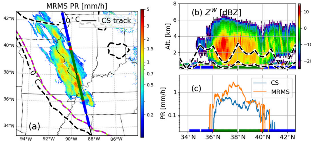
FIG. 5. (a) MRMS precipitation rates on 1918 UTC 10 Feb 2016. The thick dashed black lines mark the 2-m wet-bulb temperature isotherms of -10^{\circ}\text{C} , 0^{\circ}\text{C} , and 10^{\circ}\text{C} . The magenta–green line indicates an edge of a region where probability of snow exceeds 90% according to the methodology of Sims and Liu (2015). State boundaries are shown as dotted lines. Different colors along the CloudSat track indicate correct rejections (blue), false alarms (yellow), missed detections (red), and hits (green) of the 2C-SNOW retrieval with respect to the MRMS product. (b) The corresponding CloudSat radar reflectivity. The black–white lines mark the top and the bottom of the lowest elevation scan of the NEXRAD radars; varying heights of these lines are the result of the varying distance from the CloudSat track to the nearest ground-based radar. (c) The collocated precipitation rates from 2C-SNOW (blue) and MRMS (orange) product along the CloudSat track. The color coding at the bottom of (b) and (c) corresponds to the detection capabilities of CloudSat shown in (a). The gaps in the data correspond to the points not included in the analysis due to fractional filling, high temperature, or distance to the ground-based radars.
