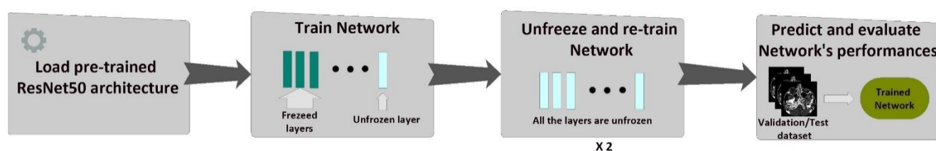
Figure 5. ResNet50 was used as a pre-trained network and, after loading the network, the fine-tuning process was started. We froze all the layers in the network except the fully-connected layers, useful for capturing high-level features on the current dataset. After the fully-connected layers have had a chance to learn patterns from our dataset, we then unfroze all the architecture layers; even the convolutional layers that had initially learned discriminative filters. We allowed each layer to be fine-tuned by performing two training steps and using differential learning rates.
