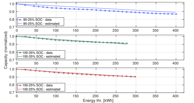
Fig. 2. Capacity vs. energy throughput: validation data for various DODs and average SOC @ T=23^\circ\text{C} , I_c=1\text{C} and I_d=1\text{C} [9].
