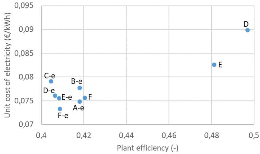
Fig. 9. Efficiency and unit cost of electricity of the examined configurations
