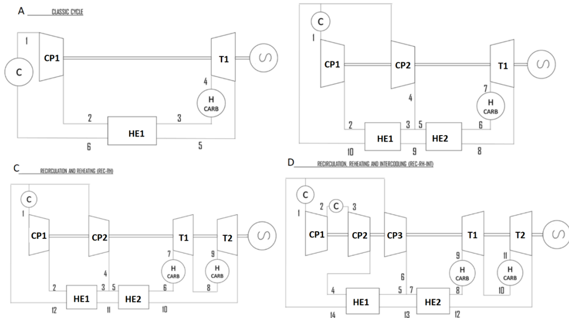
Fig. 2. Supercritical CO 2 cycles
