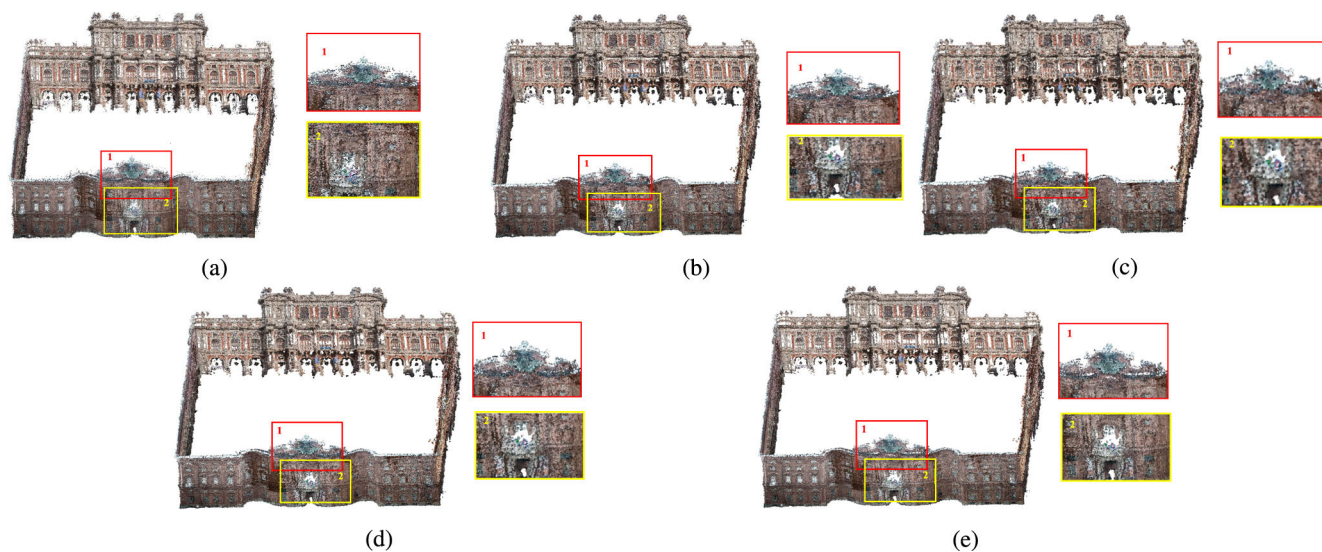
FIGURE 6. Palazzo_Carignano model. (a) Noisy input (b) outlier-free input, denoised results by (c) proposed algorithm, (d) MSGW [44] applied to outlier-free input, and (e) IBR performed after the outlier removal step [42].
