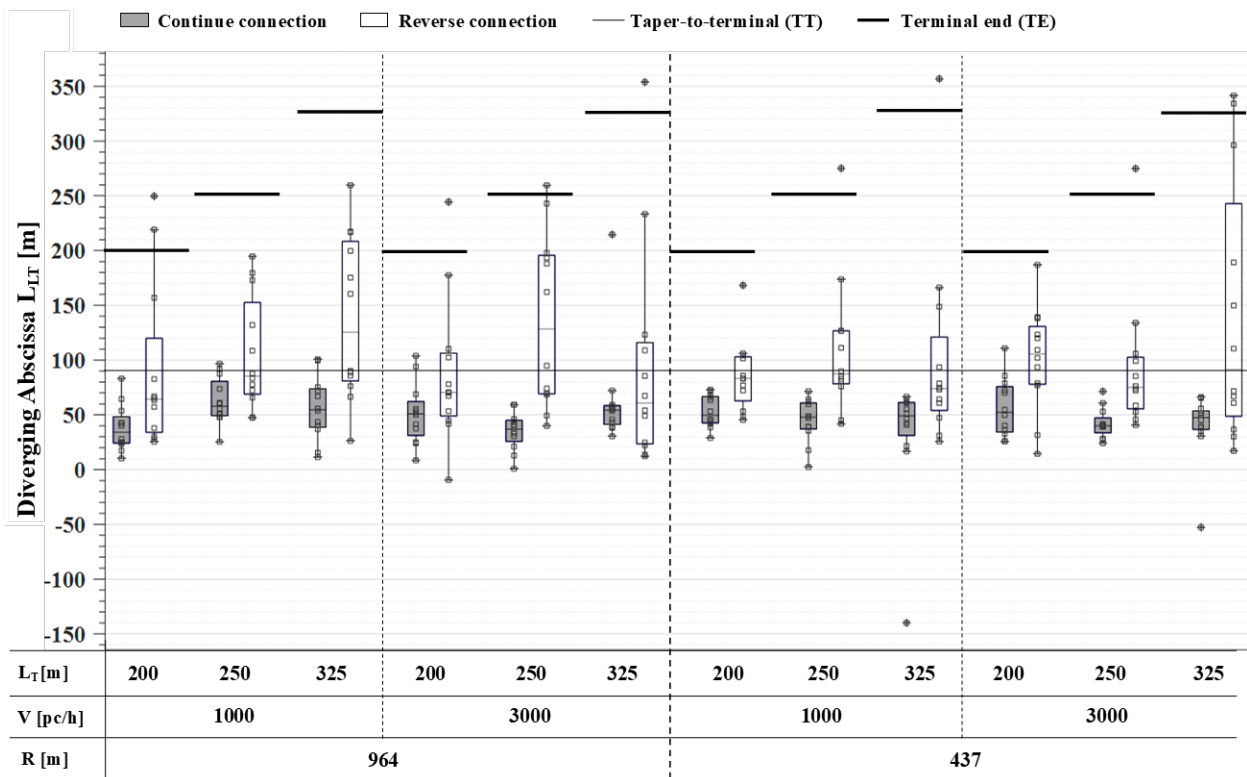
Figure 6 Abscissa of the LT section that measures the traveled path along the lane from the TS section before the lane change (Note: the thin solid line indicates the TT section, the thick solid line the TE one).
