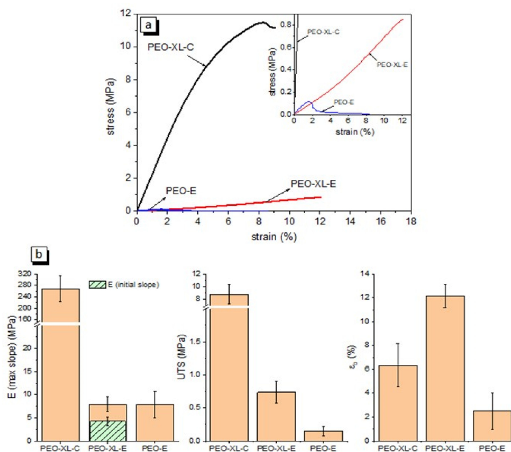
Figure 3. Results of quasi-static tensile tests. (a) Representative stress-strain curves; (b) elastic modulus ( E ), tensile strength ( UTS ), and strain at break ( \epsilon_b ) of the prepared samples (mean value and standard deviation).
