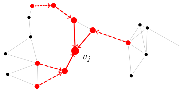
Fig. 2. A generalization of single-vertex sampling. In the graph nodes are connected only if their are closer than a certain threshold.
