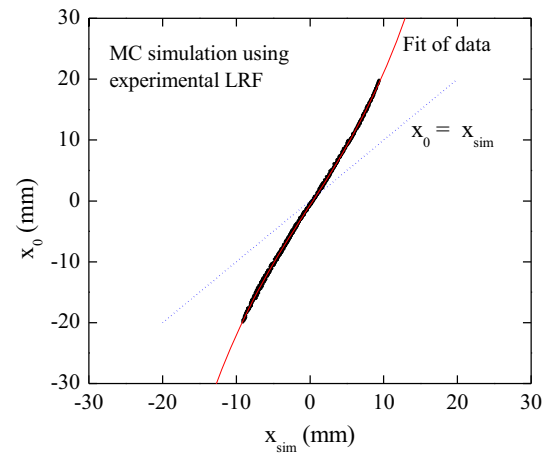
Fig. 18 Direct SiPM-matrix readout: true coordinate of interaction point x_0 as a function of reconstructed coordinate x_{sim} (black dots), the latter obtained using MC simulation with the experimental LRF , and a fit of this dependence by polynomial function (red curve). For comparison, the dependence x_0 = x_{sim} is shown (blue dotted line)
