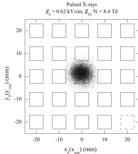
Fig. 19 Direct SiPM-matrix readout: 2D coordinate distribution of reconstructed events in x_0(x_{exp}), y_0(y_{exp}) plane. The solid boxes are the active SiPMs and the dashed box is the inactive SiPM (the photoelectron number in which was determined as the average of two adjacent channels). The data were obtained at the maximum reduced EL field, of 8.4 Td, when the detector was irradiated by pulsed X-rays through a 2 mm collimator
