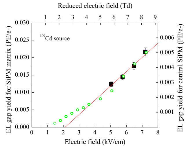
Fig. 12 Direct SiPM-matrix readout: EL gap yield for the SiPM matrix in total (solid data points, left scale) as a function of the electric field in total or reduced electric field in the EL gap, at the average energy of 82 keV deposited by gamma-rays from ^{109}\text{Cd} source in liquid Ar. The red line is a linear fit to the data points. For comparison, the EL gap yield for the central SiPM measured elsewhere [16] is shown (open data points, right scale)
