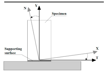
Figure 2. Misalignment errors
