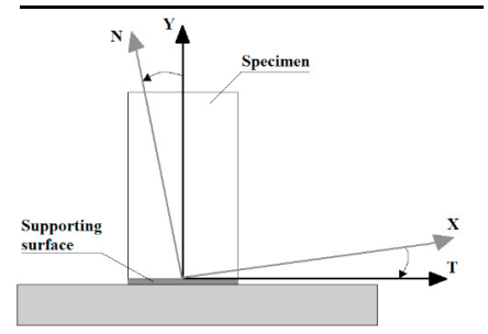
Figure 2. Misalignment errors
