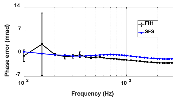
Figure 2. Phase error of the Voltage Transformer (VT) evaluated performing FH1 (square marker) and SFS (circle marker) characterization tests.
