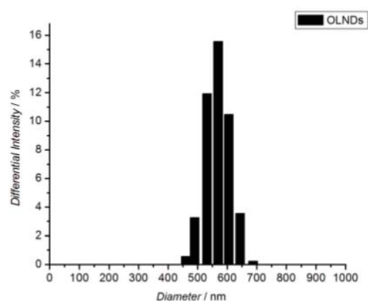
Fig. 1 Chitosan-coated OLNDs size distribution from DLS analysis
