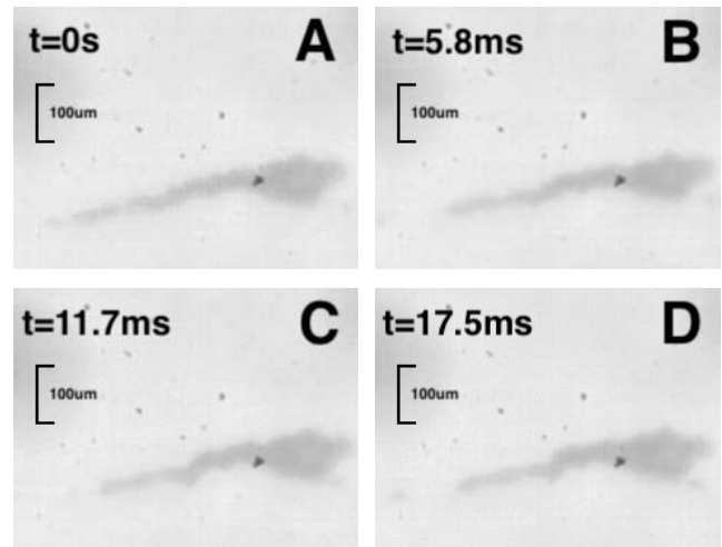
Fig. 8 Frames recorded with the high-speed camera with a frame rate of 3000 fps at different time of the PVA-coated OLNDs at acoustic pressure P_a = 74\text{MPa}
