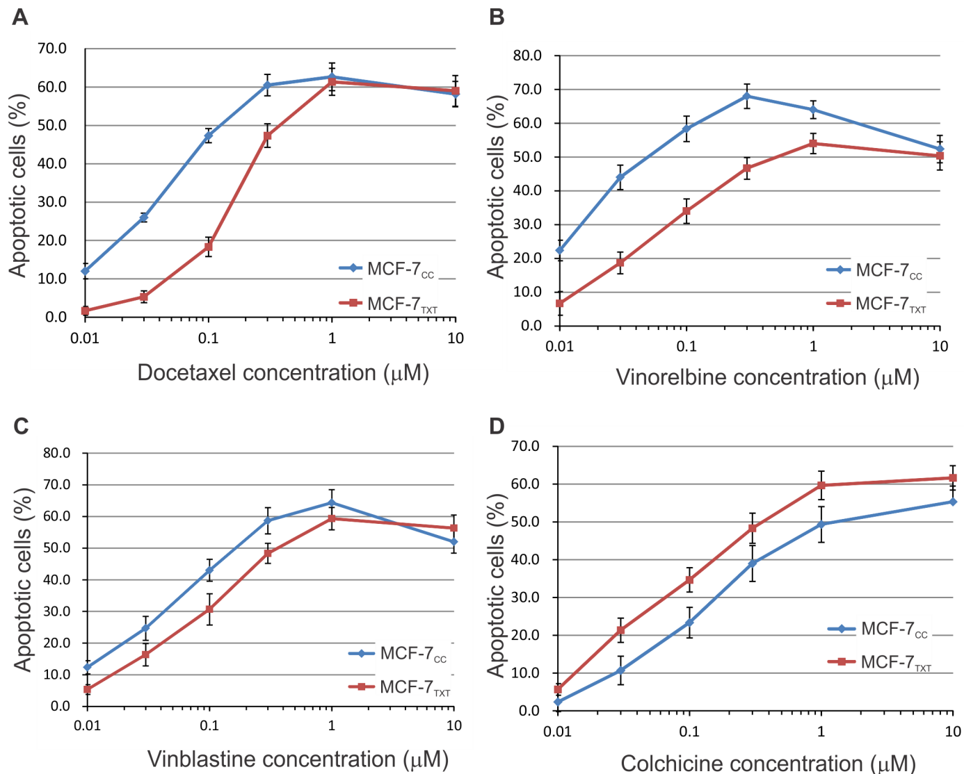
Fig 5. The effects of docetaxel, vinorelbine, vinblastine and colchicine on the apoptosis of MCF-7 CC and MCF-7 TXT cells. The apoptotic cells were determined by chromatin condensation and nuclear morphology as revealed by DAPI stain in Figs 2–4. Quantification of cell apoptosis was expressed as the percentage of the apoptotic cells of the total cells. For each data, 300 cells from at least three independent experiments were examined. Error bars are the standard errors.
