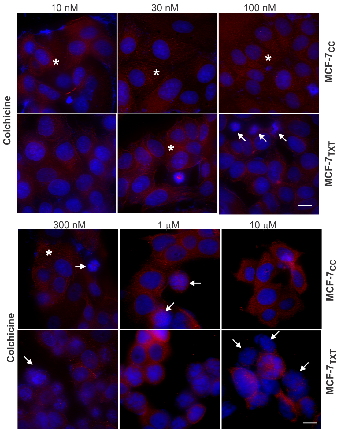
Fig 4. The effects of colchicine on the microtubule formation, M-phase arrest and cell apoptosis on the selected MCF-7 cell lines. MCF-7 CC and MCF-7 TXT cells were seeded on coverslip and treated with colchicine of indicated concentrations for 24 hours. The microtubule formation, M-phase arrest and cell apoptosis were determined by fluorescence microscopy. The red indicates the \alpha -tubulin and the blue is the DAPI stain for DNA. Size bar: 10 \mu m.
