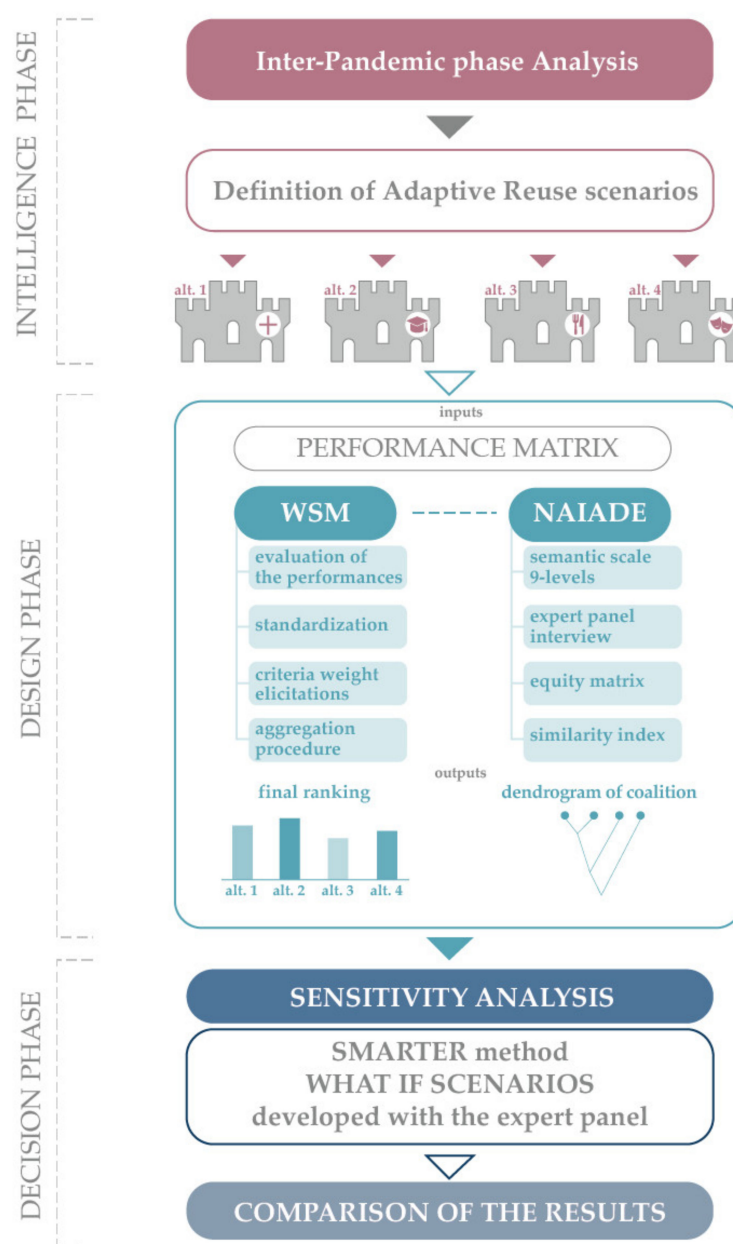
Figure 1. Methodological flowchart (where WSM: Weighted Sum Model; NAI: Novel Approach to Imprecise Assessment and Decision Environments; SMARTER: Simple Multi-Attribute Rating Technique Extended).
