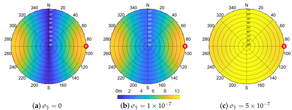
Figure 8. Analytic evaluation of \sigma_{\hat{d}} according to the position of the shared satellite and varying the magnitude of \sigma_{\hat{\gamma}} in [0, 1 \times 10^{-7}, 5 \times 10^{-7}] rad, d = 100 m, \sigma_A = \sigma_B = 7.03 m.
