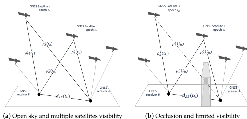
Figure 2. Pictorial representations of scenarios characterized by different visibility conditions of GNSS satellites experienced by independent receivers.
