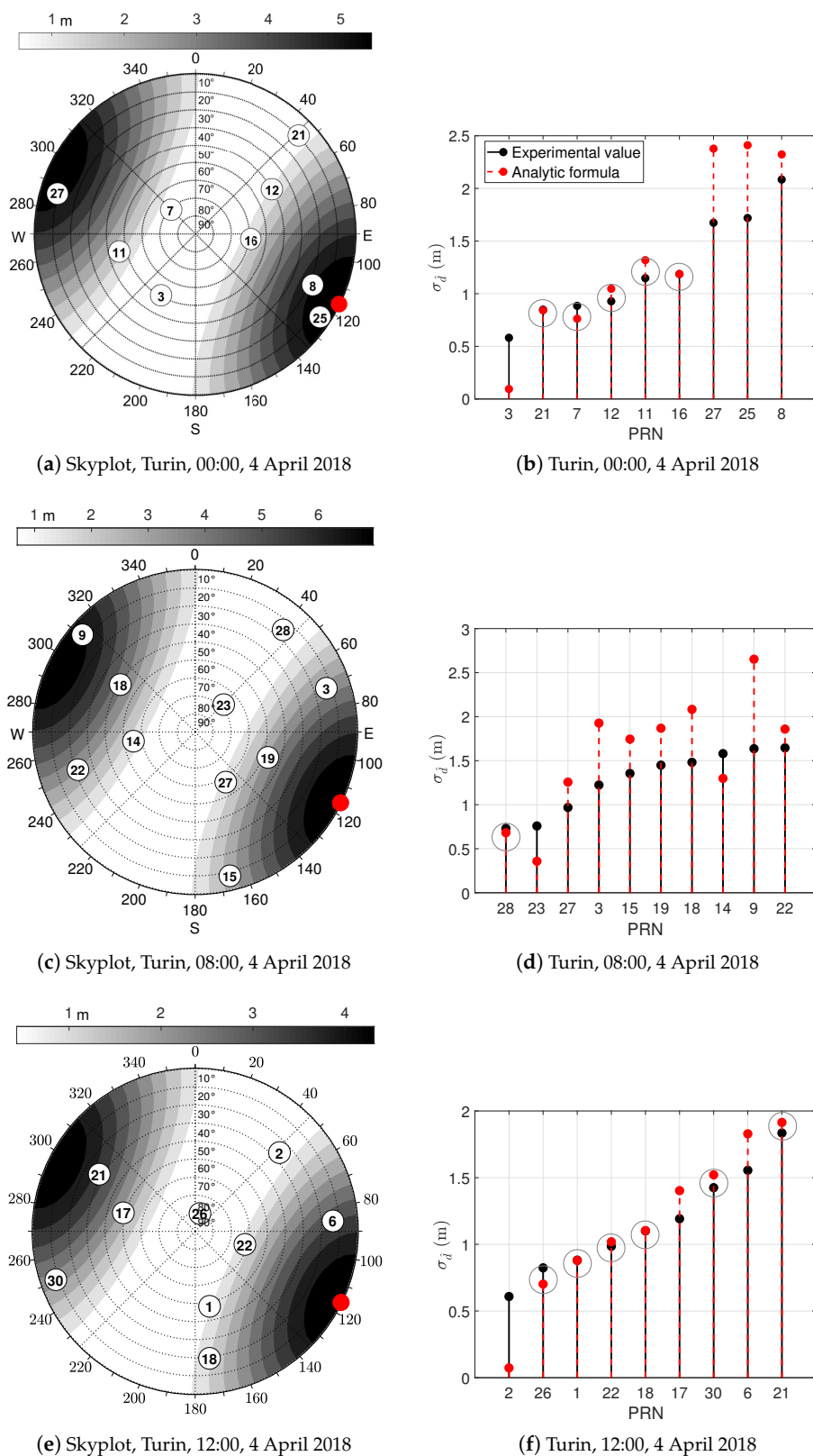
Figure 14. Skyplots (a,c,e) showing the analytic \sigma_d (color-scale) along with the superposition of satellites azimuth and elevation generated by the RFCS. Ranking plot (b,d,f) of all the shareable satellites based on the experimental standard deviation and the interpolation of the analytic model.
