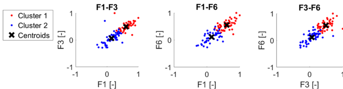
Figure 4. Clustered data (Dataset 1)
