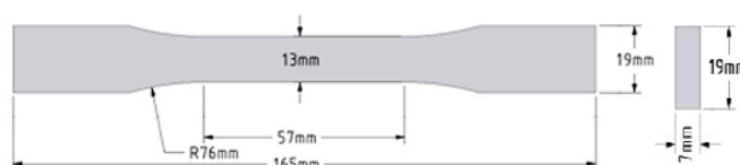
Fig. 1. Tensile test specimen's geometry and dimensions.
