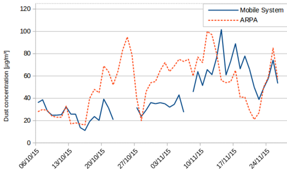
Figure 6. PM_{10} measurements at Rebaudengo Square. Lines correspond to the daily weighted mean.
