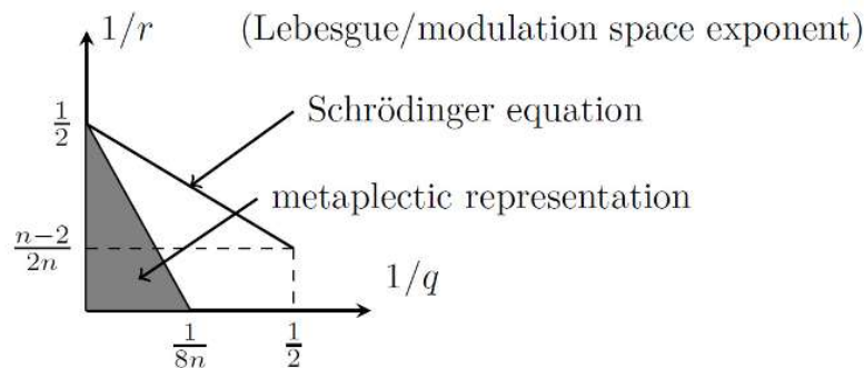
FIGURE 1. Admissible pairs for Strichartz estimates.
