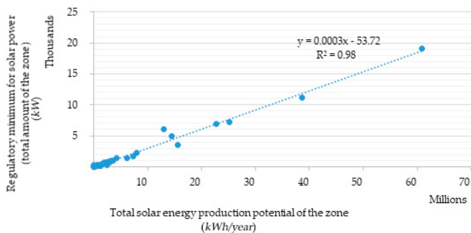
Figure 5. Regression analysis between the total solar energy production potential of the zone ( \bar{E} ) in kWh/year, and the regulatory minimum for renewable energy production in the whole zone ( \bar{P} ) in kW.
