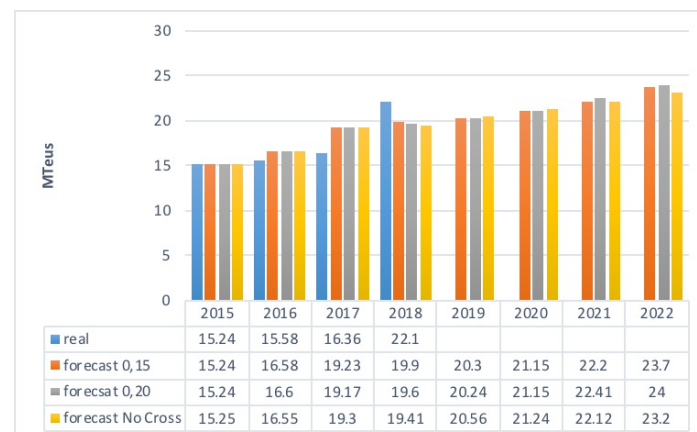
Fig. 7. Port available real capacity vs simulation forecast
