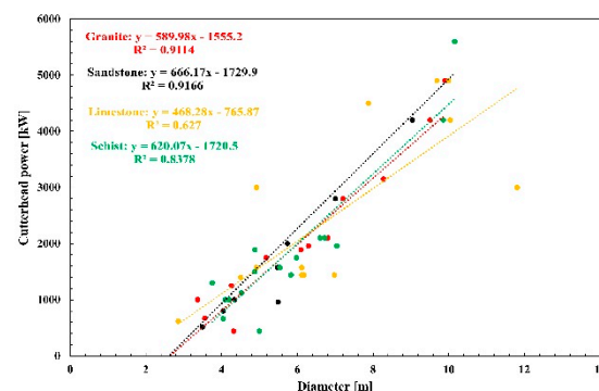
Figure 17. Correlation between the diameter and the power due to the excavation in granite, sandstone, limestone, and schist by double shield TBMs.
